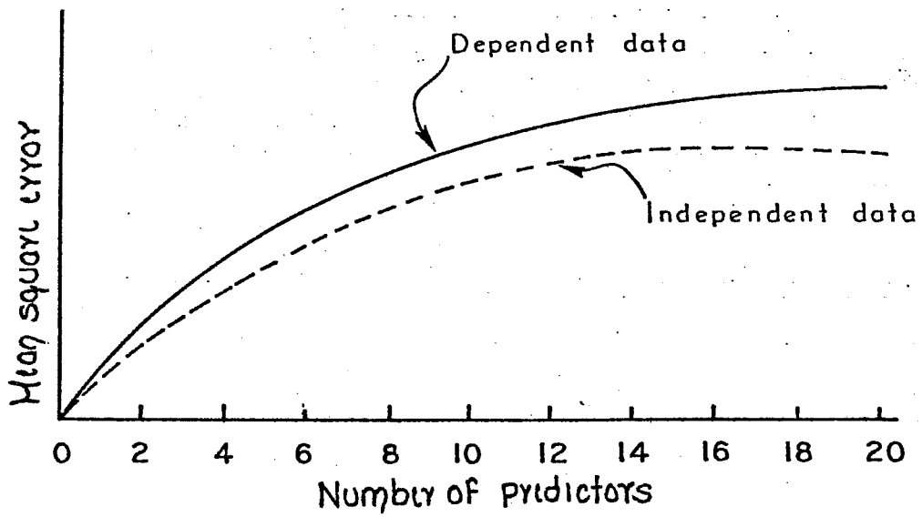
Figure 5. Schematic diagram of mean square error as a function of number of predictors.
