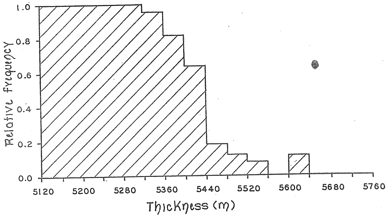
Figure 2. Relative frequency of frozen precipitation at Salt Lake City, Utah, as a function of forecast 1000-500 mb thickness (after Glahn and Bocchieri, 1975).
